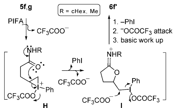
Scheme 4. Proposed mechanism for the transformation of amides 5f,g into lactone 6f' .
