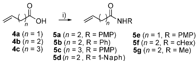
Scheme 1. Preparation of linear unsaturated amides 5a–g . Reagents and conditions : i) (a) (COCl) 2 , CH 2 Cl 2 , room temperature; (b) RNH 2 , pyridine, CH 2 Cl 2 , room temperature (87% for 5a ; 82% for 5b ; 98% for 5c ; 80% for 5d ; 72% for 5e ; 78% for 5f ; 64% for 5g ).
