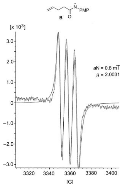
Figure 2. EPR spectrum of the amidyl radical B .
