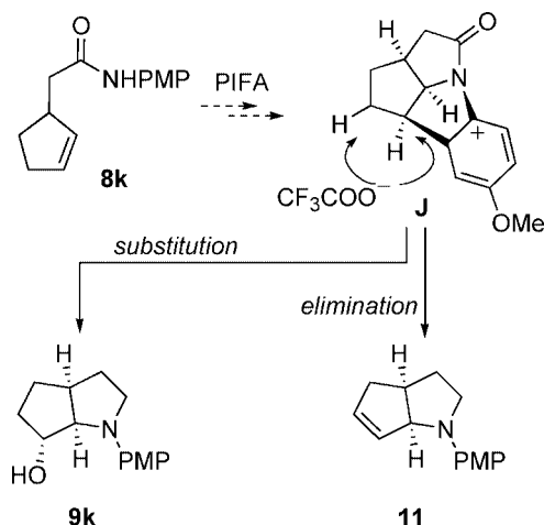
Scheme 5. Proposed mechanism for the formation of bicycles 9k and 11 .
