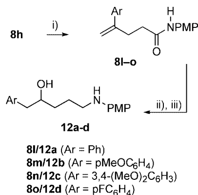
Scheme 7. Synthesis and reactivity of 4-aryl-substituted \gamma,\delta -unsaturated amides 8l–o . Preparation of amino alcohols 12a–d . Reagents and conditions: i) ArB(OH) 2 , Pd(PPh 3 ) 4 , K 2 CO 3 , DMF/H 2 O, 50 °C (63% for 8l ; 63% for 8m ; 52% for 8n ; 61% for 8o ); ii) PIFA, CF 3 CH 2 OH, 0 °C; (iii) BH 3 ·SMe 2 , THF, 0 °C \rightarrow room temperature (37% for 8l ; 65% for 8m ; 83% for 8n ; 20% for 8o ).
