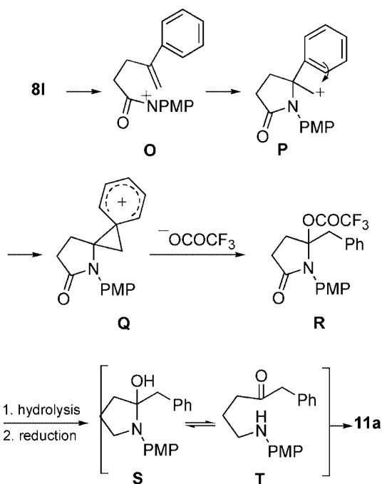
Scheme 8. Proposed mechanism for the transformation of amides 8l–o into amino alcohols 12a–d .
