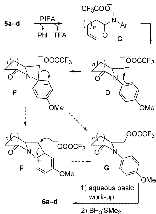
Scheme 3. Proposed mechanism for the intramolecular olefin amidohydroxylation.
