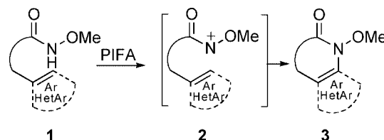
Figure 1. Intramolecular reaction of (hetero)aromatic rings with N -acylnitrenium ions generated by PIFA.
