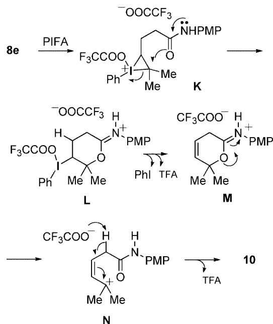
Scheme 6. Proposed mechanism for the formation of diene 10 .
